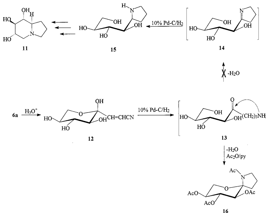
Scheme 4. Cyclization of 12 to spiroaminoketal 16
