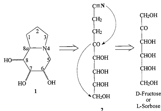
Scheme 1. Retrosynthesis of 1
