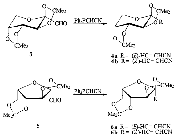
Scheme 2. Formation of 4-octulosononitrile derivatives by Wittig methodology
