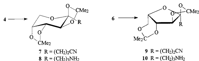
Scheme 3. Synthesis of 1-amino-1-deoxy-4-octulose derivatives
