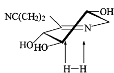
Figure 1. Stereochemical course for the hydrogenation of 25
