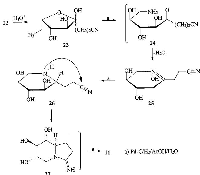
Scheme 6. Double cyclization of 22 to 1-deoxycastanospermene ( 11 )
