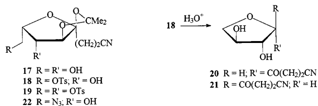
Scheme 5. Formation of 5,8-anhydro-4-octulosononitrile derivatives ( 20 and 21 ) from 18
